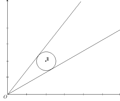
Figure 19: A section along the first diagonal along the line containing the origin O and \mathbb{1} of the LH-ellipticity domain of the energy function F \mapsto e^{\|\text{dev}_3 \log U\|^2} if it is LH-elliptic in a ball.
