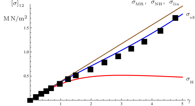
Figure 11: The shear stress \sigma_{12} corresponding to the amount of shear \gamma for the energies W_{\text{eH}} , W_{\text{H}} , the Neo-Hooke energy W_{\text{NH}} , the Mooney-Rivlin energy W_{\text{MR}} and the infinitesimal case corresponding to rubber: \mu = \frac{E}{2(1+\nu)} = 0.39 \text{ MN/m}^2 (according to Treloar's data [248]). For the exponentiated energy W_{\text{eH}} we have chosen \frac{3}{16} < k = 0.243 . The squares (■) represent the experimental data for the simple shear deformation of vulcanized rubber, measured in 1944 by L.R.G. Treloar [247] and in 1975 by L.R.G. Treloar and D.F. Jones [124] (see also [248, 249]) and provided by courtesy of R. Ogden, in the form of tab-separated ASCII-files (see [246]).
